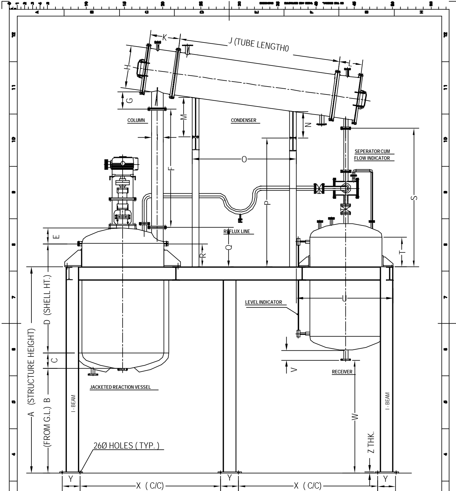
STRUCTURE LAY OUT (FRONT - VIEW)
